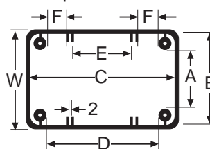
Top View UB5
