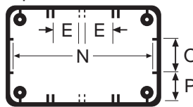
Top View UB1, UB2
